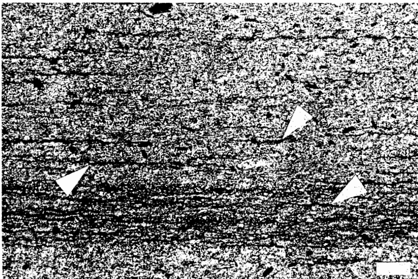
Figure 9.8. Photomicrograph of ML-3 (Prichard Formation) showing massive clayey shale bed with gradual variation in the amount of carbonaceous flakes (arrows). These gradual variations are interpreted to indicate fluctuations in sediment supply during background sedimentation. Scale bar is 200 \mu\text{m} .
