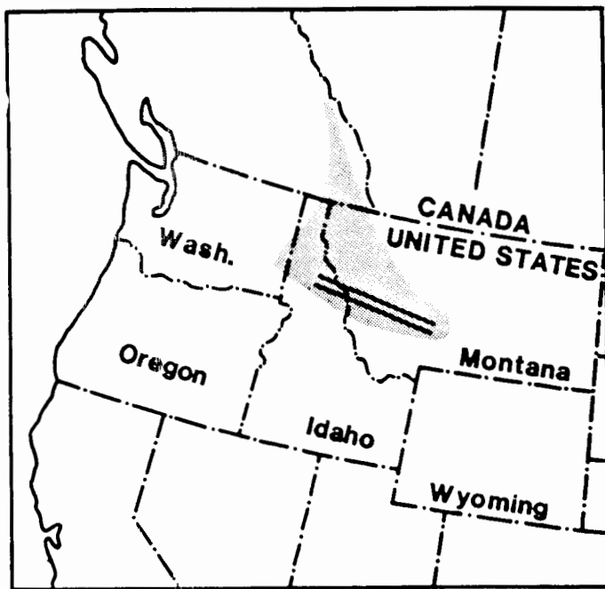
Figure 9.1. Location map. Stipple pattern shows present day outline of the Belt basin. Newland shale samples were collected from the eastern extension of the basin, Prichard and Aidridge shale samples were collected from the central, western, and northwestern portion of the basin. The pair of solid lines indicates the approximate position of the east-west slice shown in Figure 9.3.
