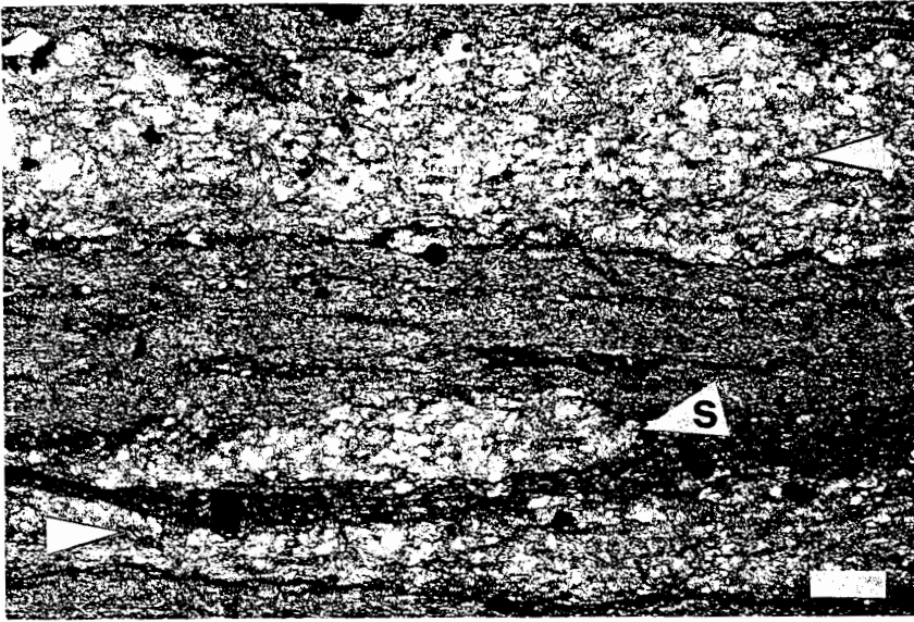
Figure 9.7. Photomicrograph of ML-2 (Prichard Formation) showing wavy-lenticular silt laminae with sharp boundaries (arrows), and single silt lens (arrow labeled S). Scale bar is 200 \mu\text{m} .
